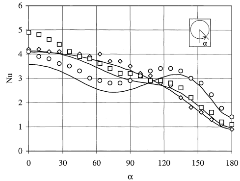
Fig. 10. Calculated and experimental local Nusselt number distribution in the cylinder surface at Ra 3.4 \times 10^3 : (○) W^* = 2.1 , (□) W^* = 2.9 and (◇) W^* = 3.6 .
