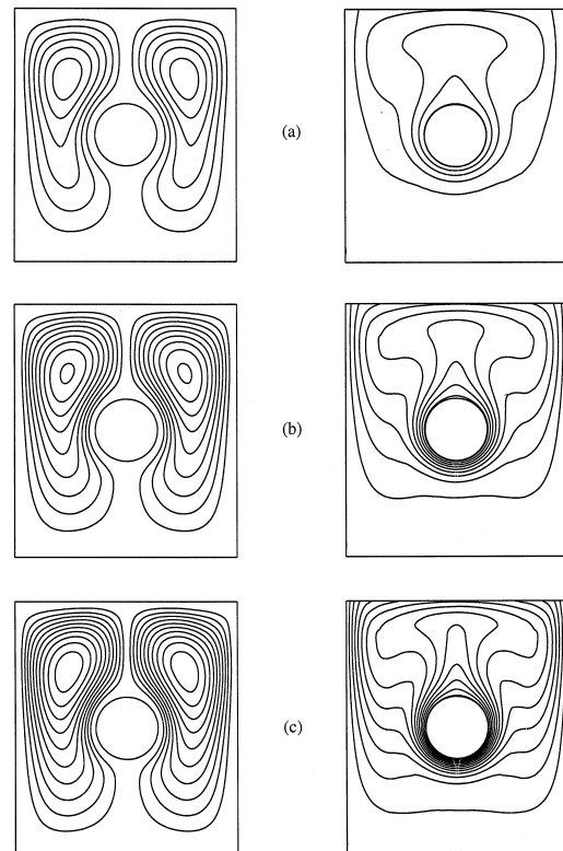
Fig. 6. Calculated streamlines ( -2.5 \times 10^{-3} ( 0.25 \times 10^{-4} ) 2.5 \times 10^{-3} ) and temperature (1 K) distributions in the W^* = 3.6 cavity: (a) Ra = 1.3 \times 10^3 , (b) Ra = 2.4 \times 10^3 and (c) Ra = 3.4 \times 10^3 .
